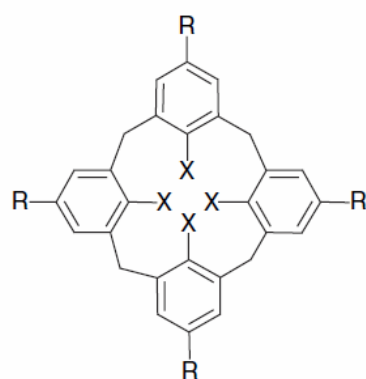
Calix[4]arene
